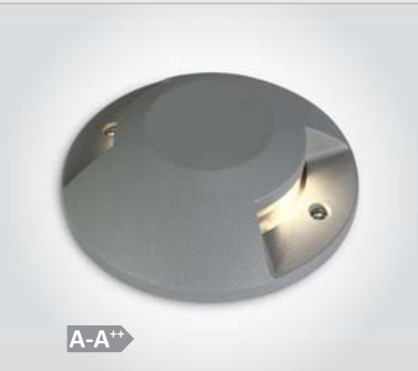
69058B | 2x6W | COB LED | Die cast
